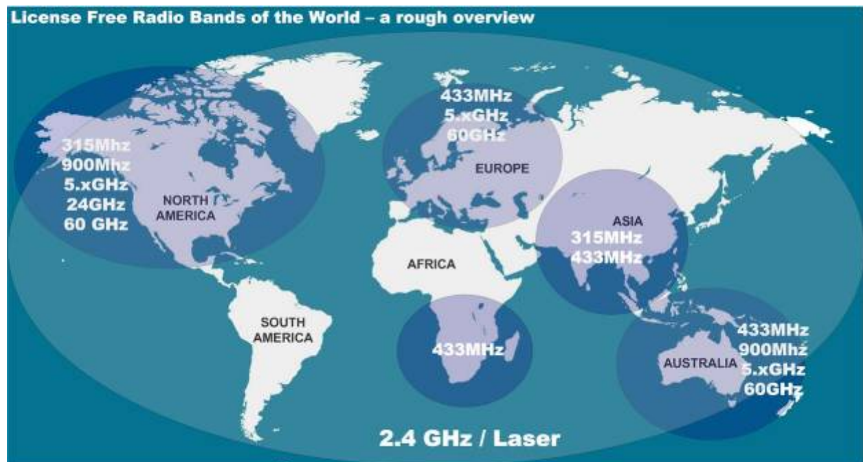
Figure 1. License Free Bands of the World – a rough overview
